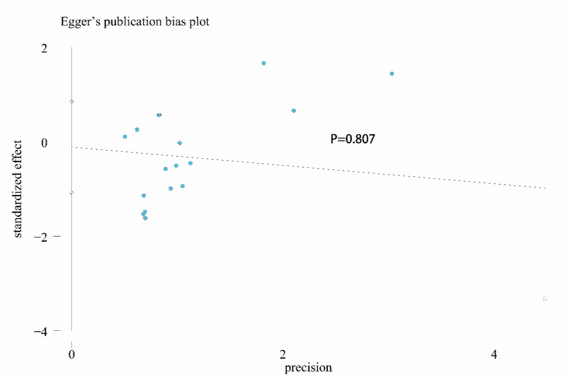
eFigure 5. Funnel plots (left) and Egger's test (right) of treatment for 12-16 weeks in (A) PGA 0/1, (B) PASI-75, (C) TEAEs and (D) DAE;
