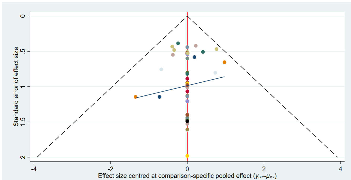
eFigure 5. Funnel plots (left) and Egger's test (right) of treatment for 12-16 weeks in (A) PGA 0/1, (B) PASI-75, (C) TEAEs and (D) DAE;
